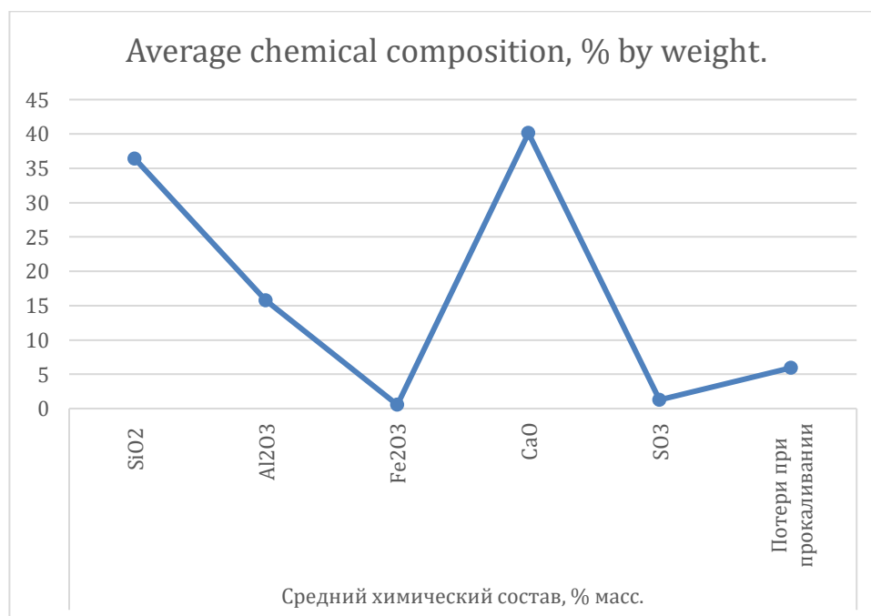
Graph 1. Chemical composition of blast furnace slag (data taken from [9])
