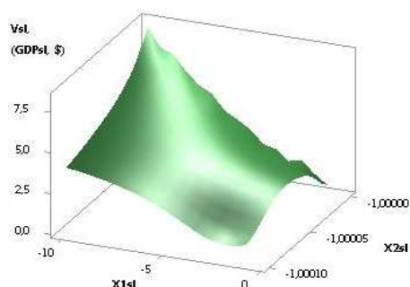
Fig. 5. 3D of Vsl (GDPsl)
