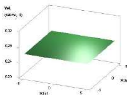
Fig. 4. 3D of Vsl (GDPsl)
