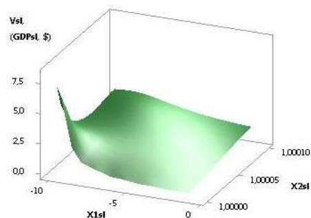
Fig. 6. 3D of Vsl (GDPsl)
