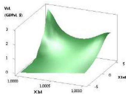
Fig. 2. 3D of Vsl (GDPsl)
