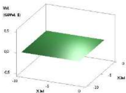
Fig. 3. 3D of Vsl (GDPsl)
